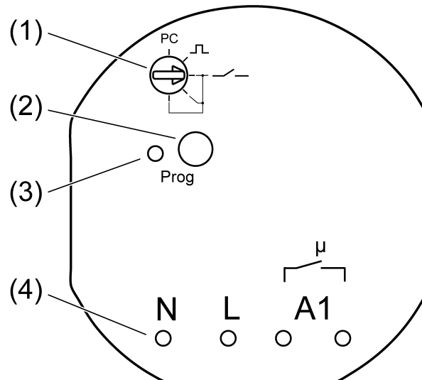
Figure 2: Radio switching/push-button actuator potential-free
