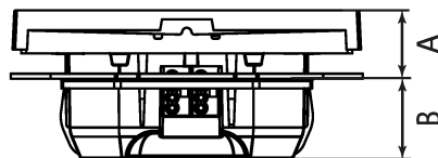
Figure 11: Installation dimensions
