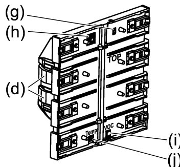
Figure 4: Push-button sensor
