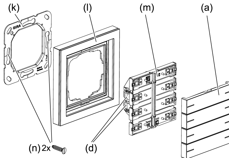
Figure 5: Mount device
