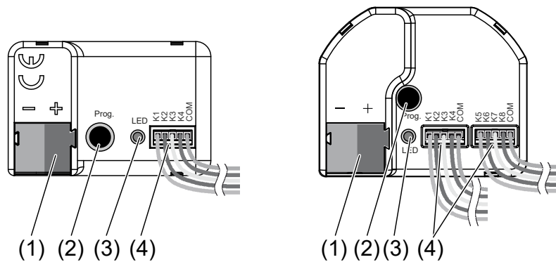
Figure 1: Device components
