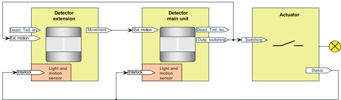
Figure 40: Application example with twilight level evaluation in the main unit and extensions for output function "Staircase function"
