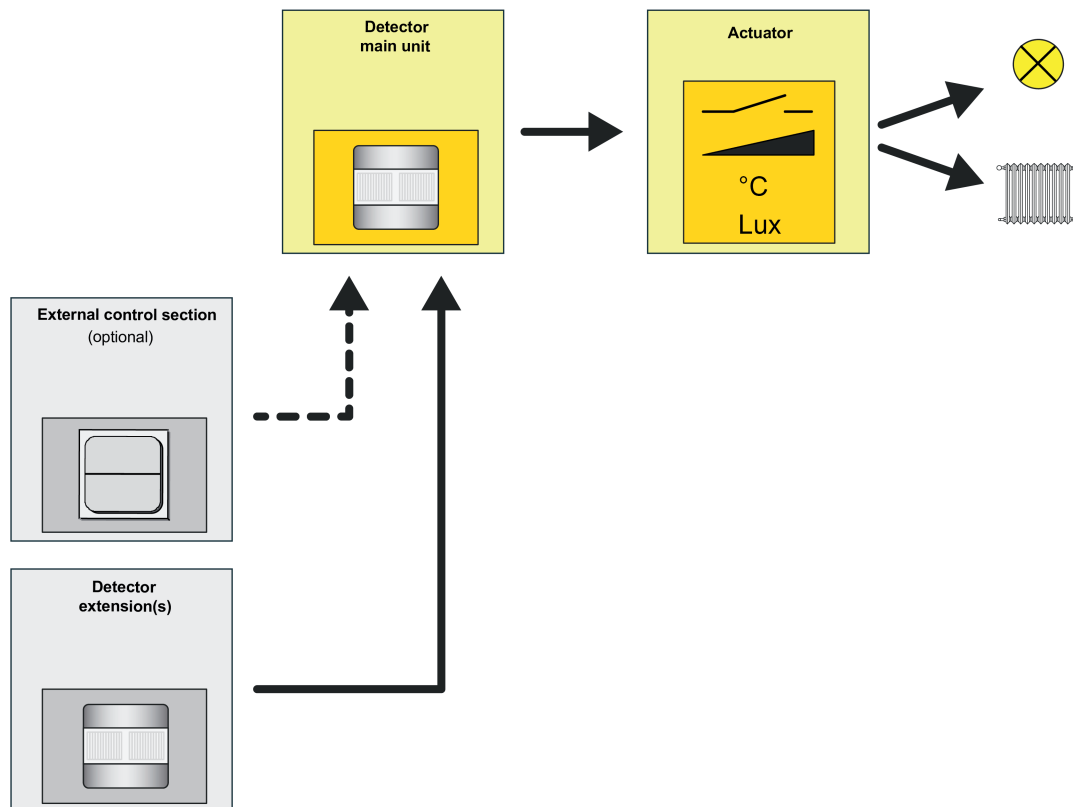
Figure 29: Application type "Main unit"
