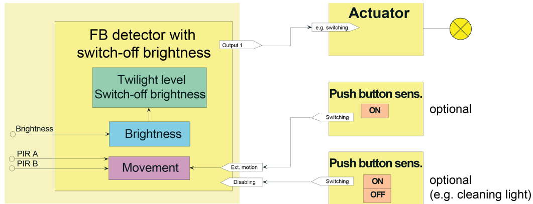
Figure 25: Application example of the application Detector with switch-off brightness
