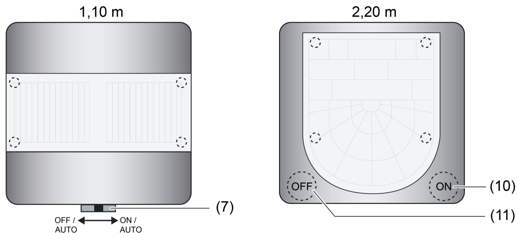
Figure 32: Arrangement of the operating elements for local operation (operating mode switchover)
