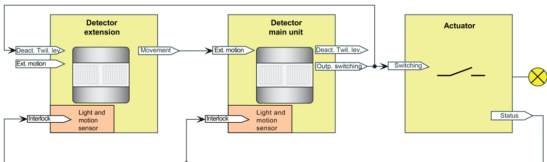
Figure 38: Application example with twilight level evaluation in the main unit and extensions for the data format "Switching"
