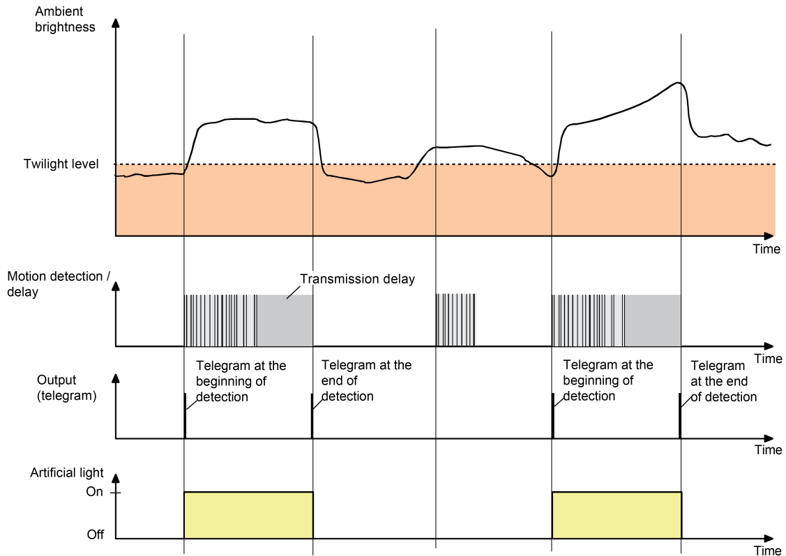
Figure 24: Brightness and motion evaluation with the detector
