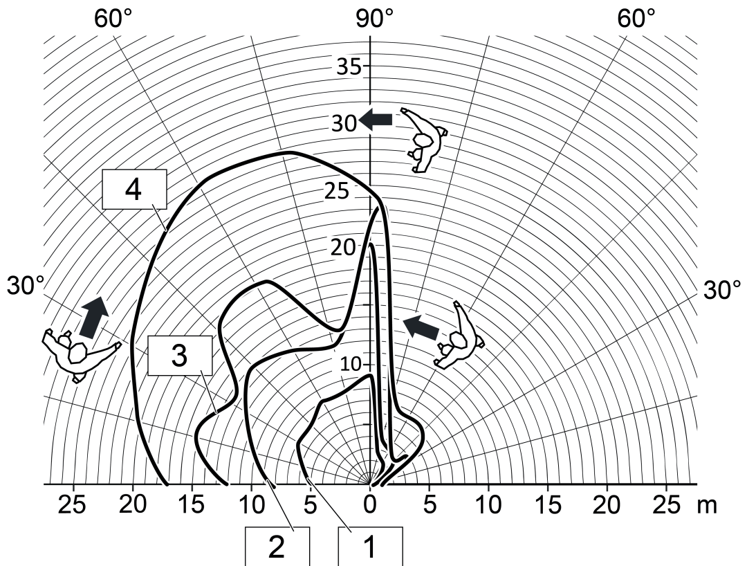
Figure 13: Range with tangential direction of motion, device variant 1.10 m, only one sensor active
