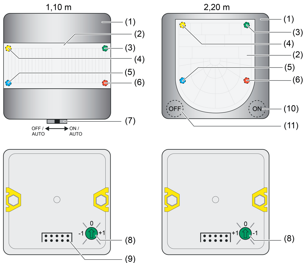
Figure 1: Device components Top: Front side / Bottom: Rear side
