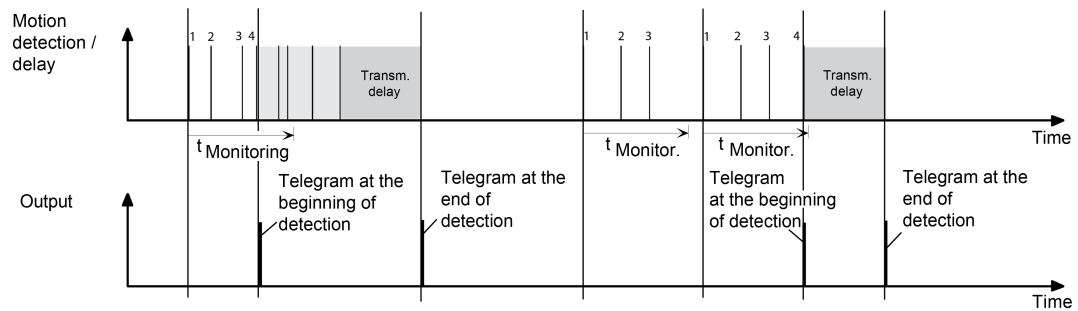
Figure 27: Motion evaluation with the detector
