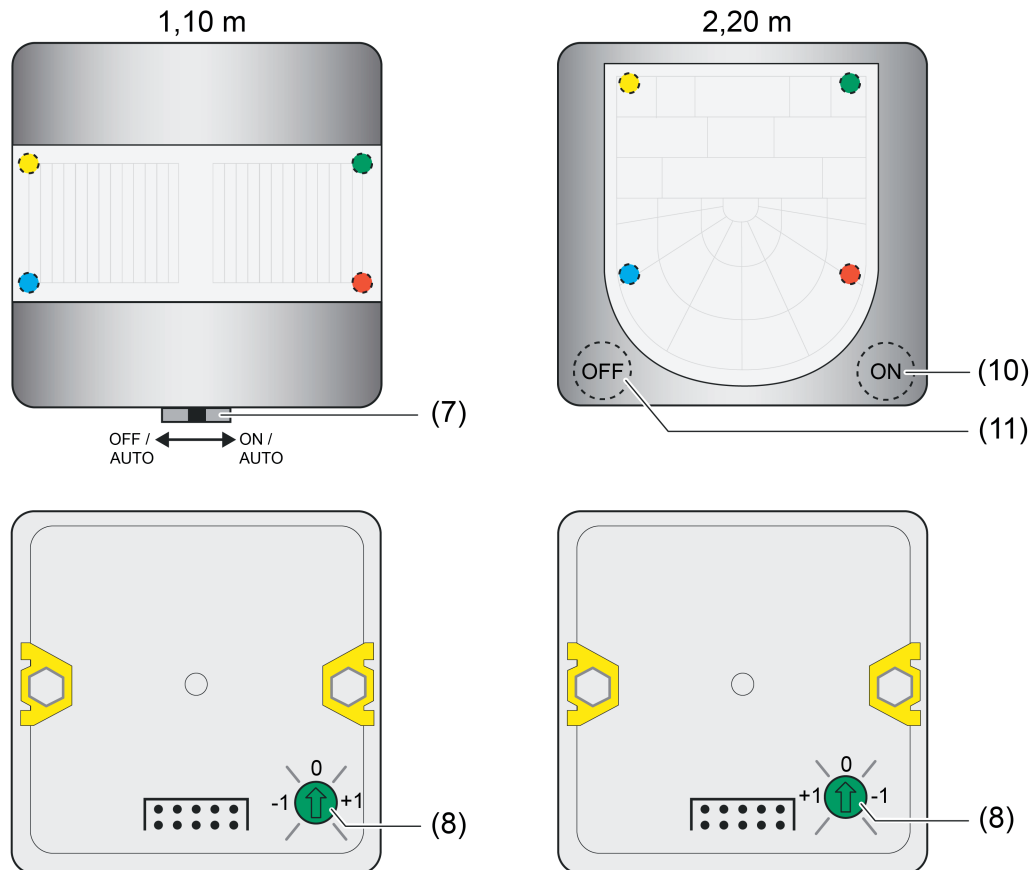
Figure 18: Operating elements on the device
