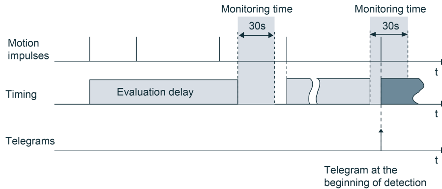
Figure 46: Evaluation delay with only brief motion
