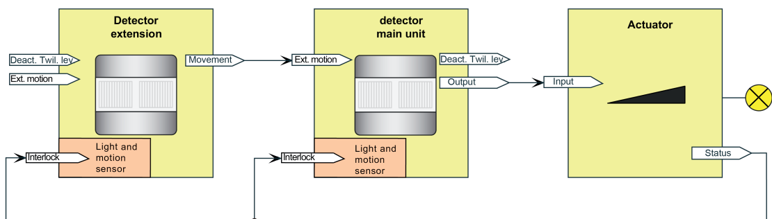
Figure 37: Application example of main unit and extension with twilight level evaluation in the main unit
