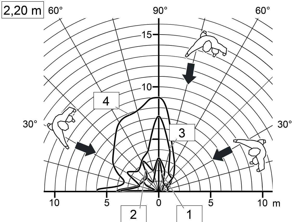
Figure 16: Range with radial direction of motion, device variant 2.20 m, mounting height 2.20 m, only one sensor active
