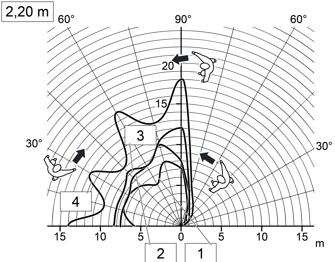
Figure 15: Range with tangential direction of motion, device variant 2.20 m, mounting height 2.20 m, only one sensor active
