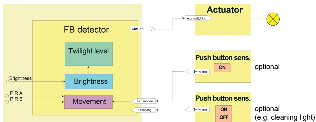
Figure 23: Application example of the application detector
