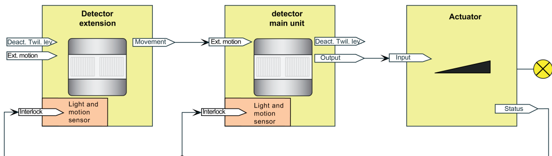
Figure 36: Application example of main unit and extension without twilight level evaluation
