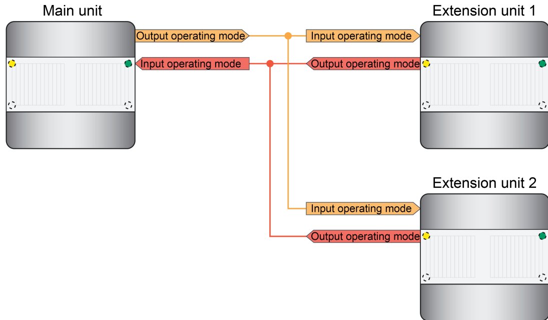
Figure 34: Example of the linking of a main unit with two extensions for operating mode switchover and display
