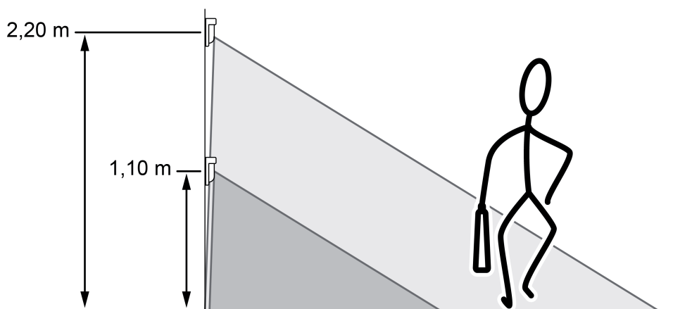
Figure 9: Detection field and mounting height
