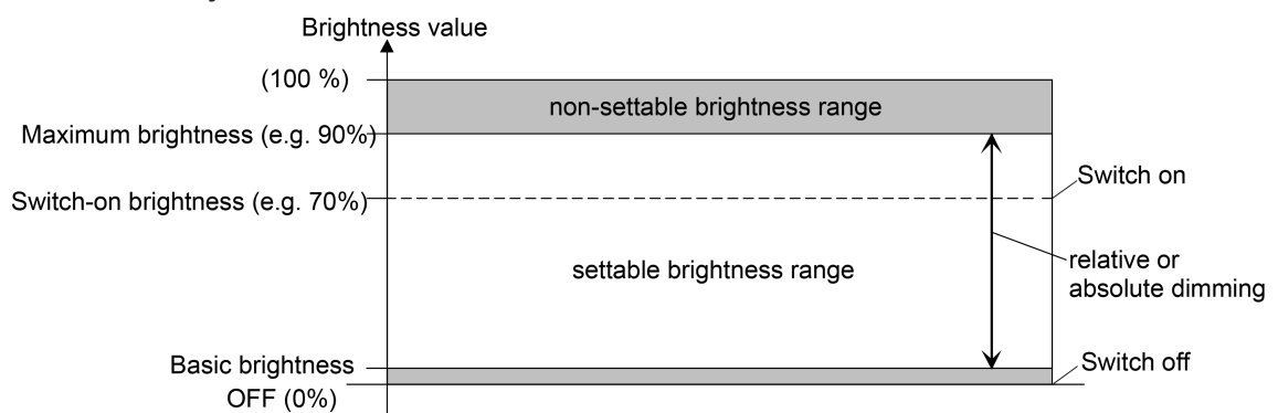
Image 9: Example of a brightness range with basic brightness
