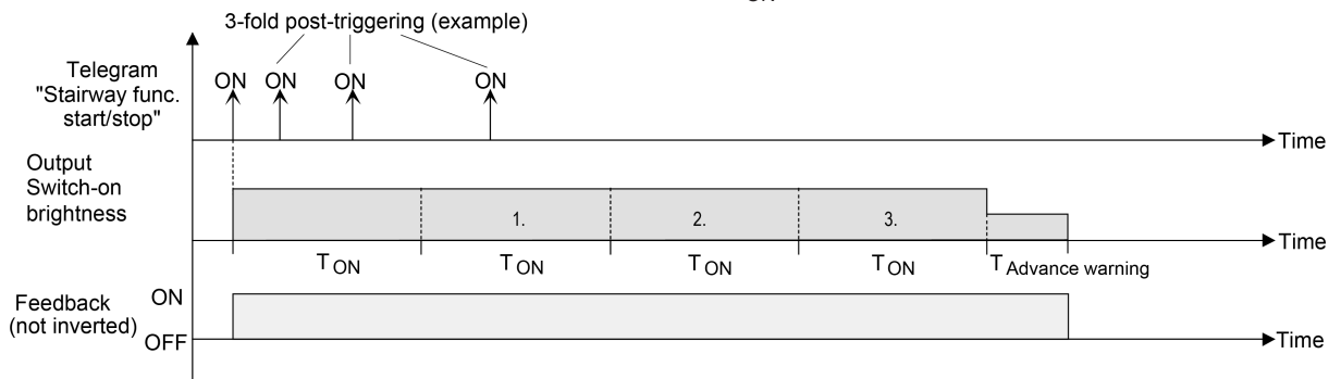
Image 22: Time extension of the staircase function
