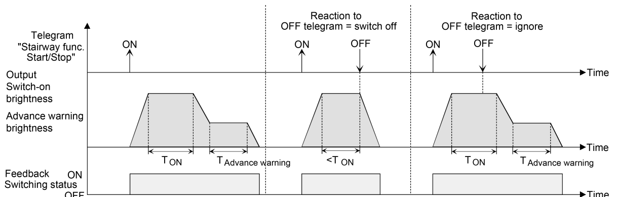
Image 17: Switch-off behaviour of the staircase function with soft functions (as an example with minimum brightness = 0 %)
