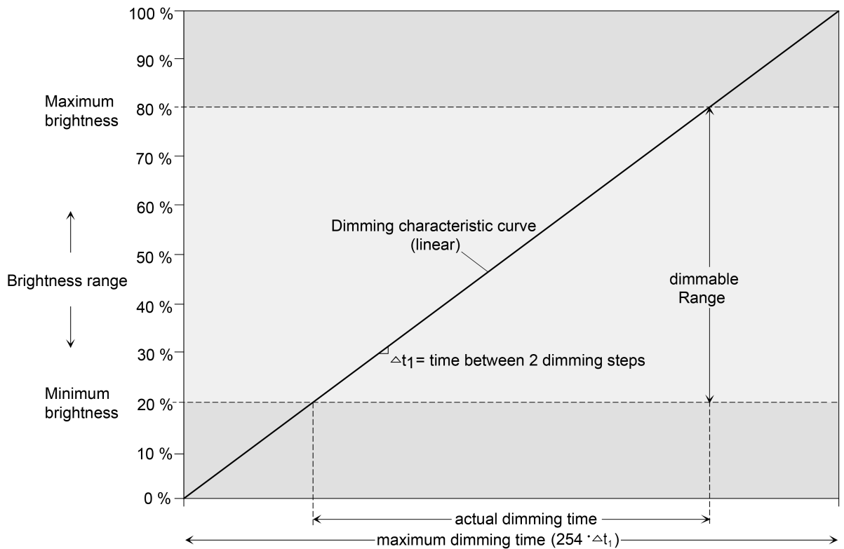
Image 6: Linear characteristic dimming curve as an example with minimum brightness > 0 % and maximum brightness
