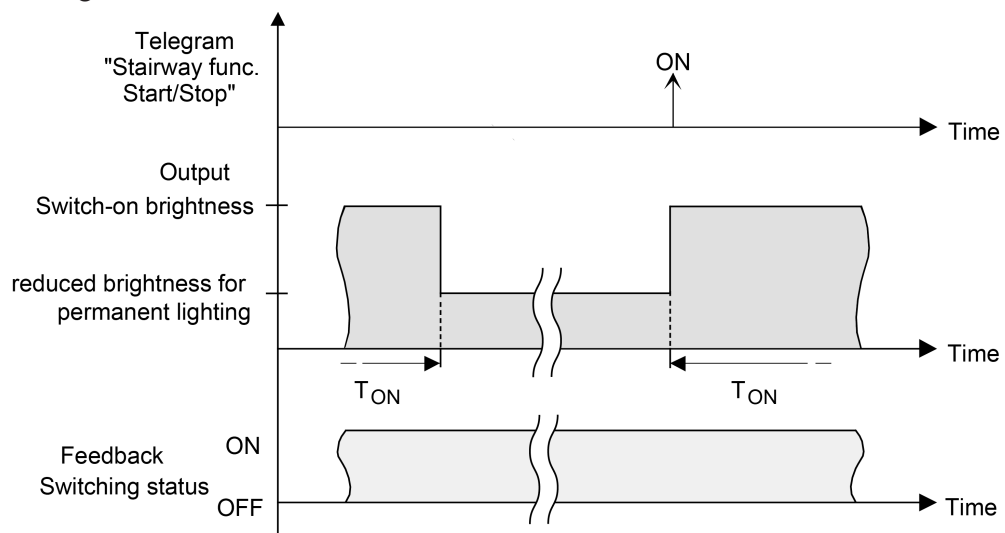
Image 20: The continuous lighting of the staircase function without soft functions
