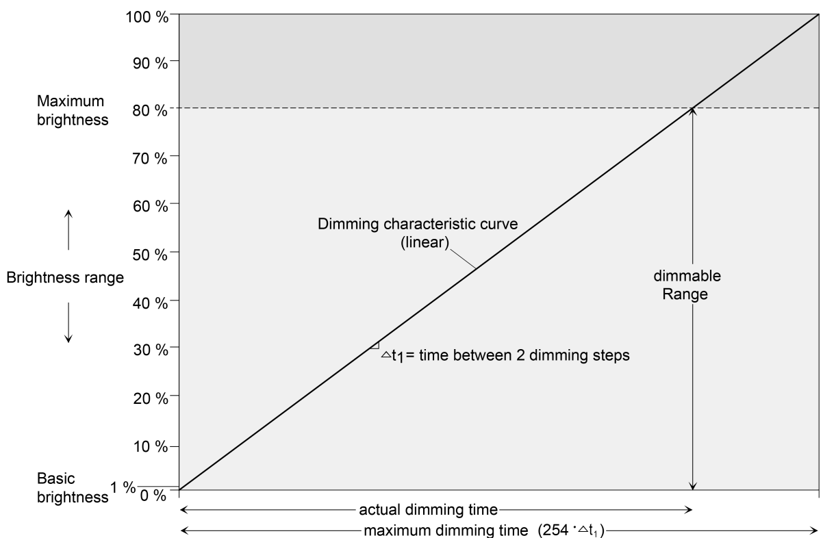
Image 5: Linear dimming characteristic as an example with basic brightness and maximum brightness
