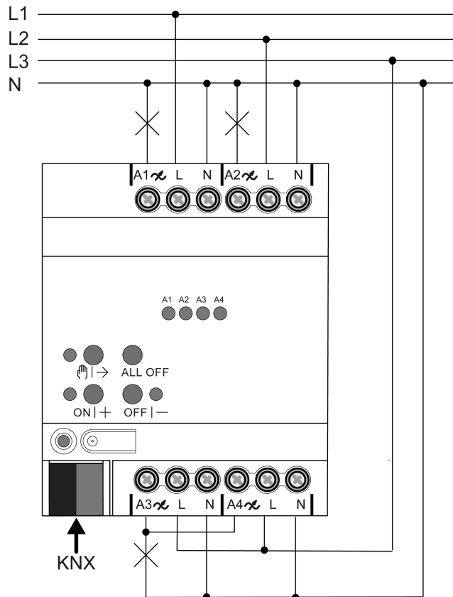
Image 2: Comfort variant of the device connection with dimmer outputs switched in parallel (connection example)
