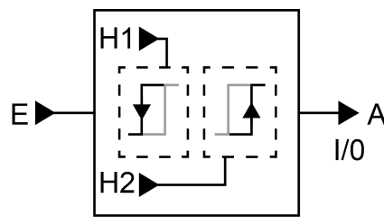
Image 29: Limit value switch
