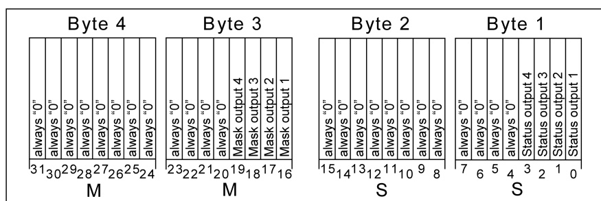
Image 11: Object structure "23" of the collective feedback for outputs 1 ... 4
