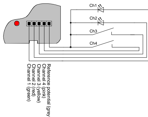
Example of push button interface used with 2 inputs and 2 outputs
