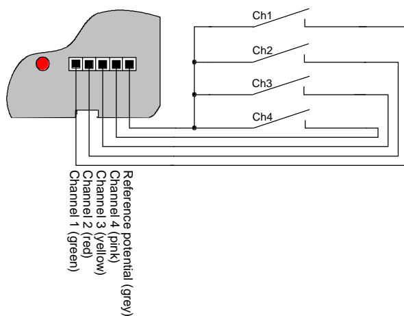
Push button interface used as 4 inputs
