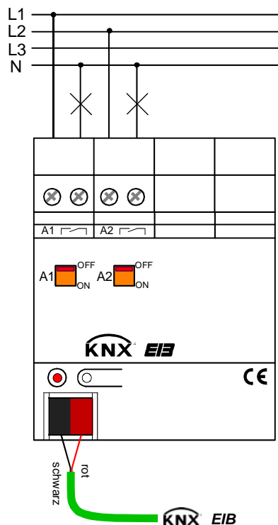
Fig. 1: Electrical connection
